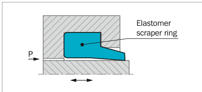
Figure 186: Scraper WRM
