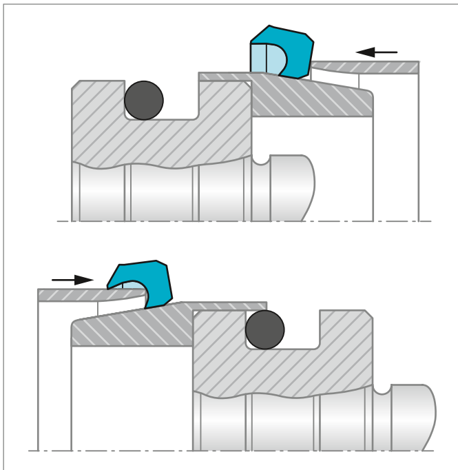
Figure 104: Installation of Piston VL Seal® in closed groove
