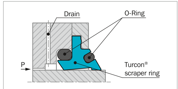
Figure 173: Optional Turcon® Excluder® SR with O-Ring activated Excluder® lip
