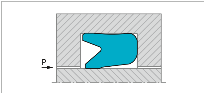
Figure 52: U-Cup, type RU9
