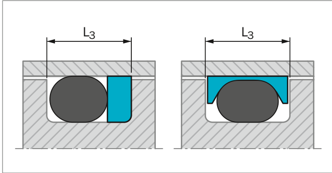
Figure 133: Groove width
