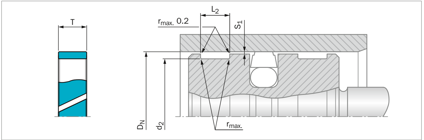
Figure 205: Piston guide
