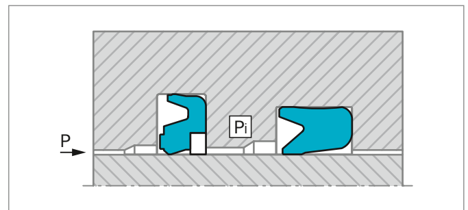
Figure 60: Tandem configuration
