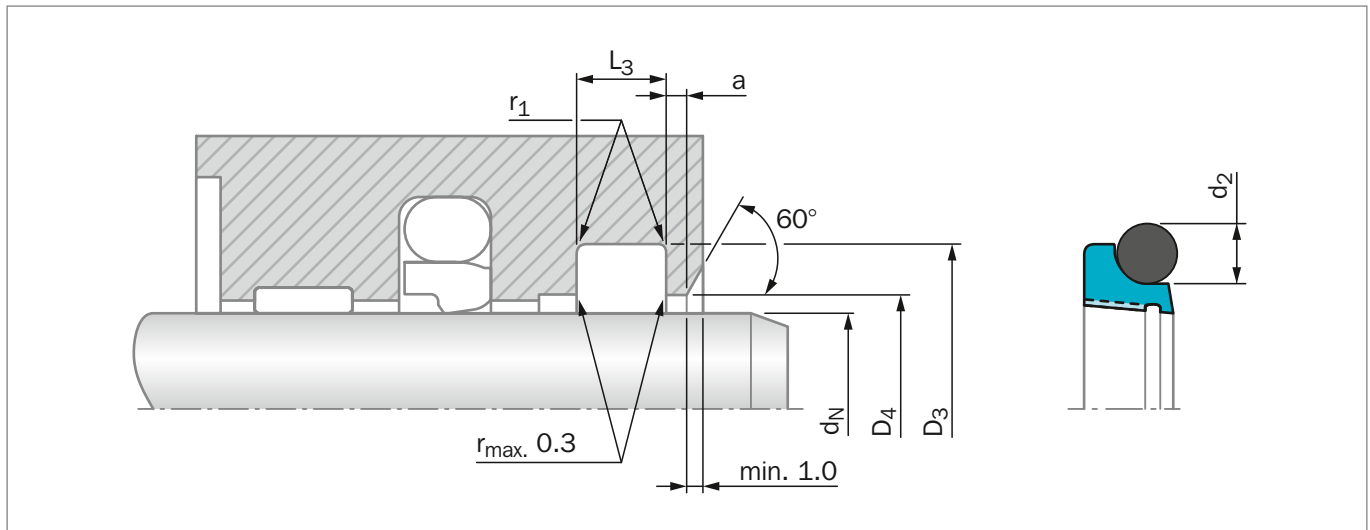
Figure 178: Installation Drawing
