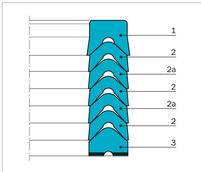
Figure 35: Veepac design
