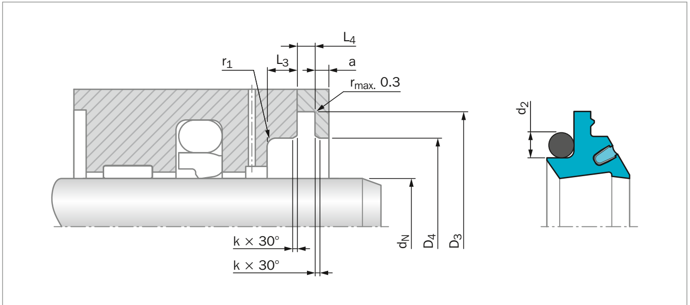
Figure 171: Installation Drawing
