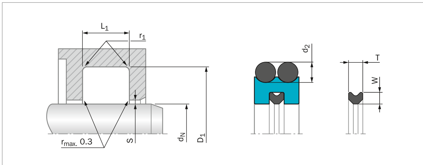
Figure 87: Installation Drawing
