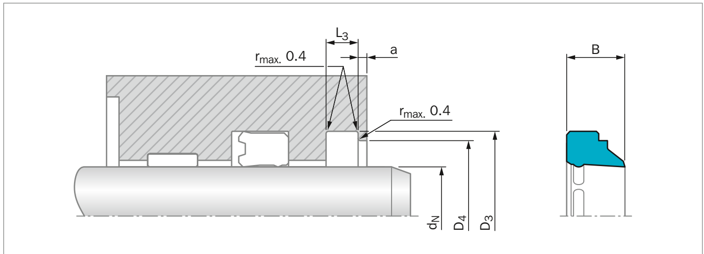
Figure 189: Installation Drawing
