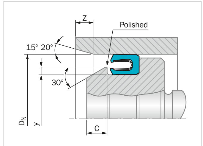
Figure 105: Installation in a half-open groove
