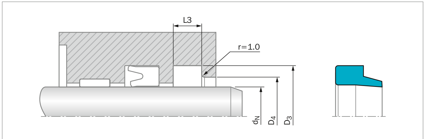
Figure 187: Installation Drawing
