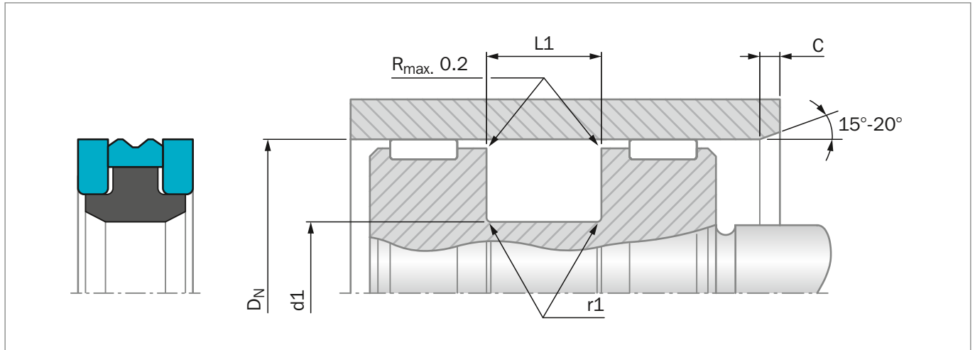
Figure 149: Installation Drawing
