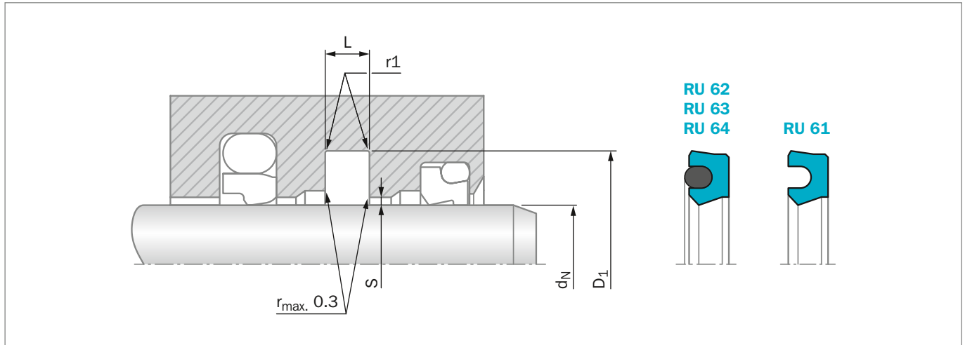
Figure 51: Installation Drawing
