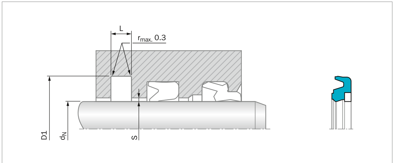
Figure 65: Installation Drawing
