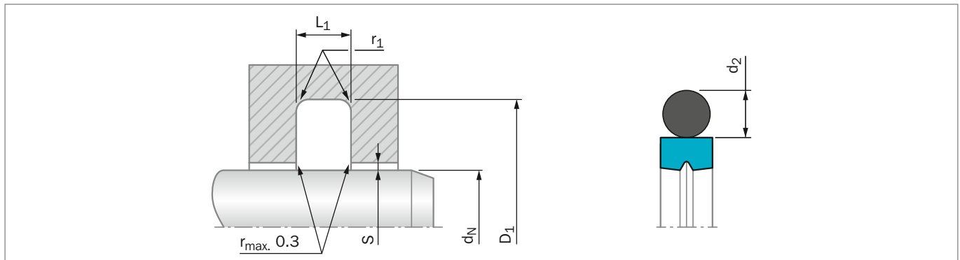
Figure 83: Installation Drawing
