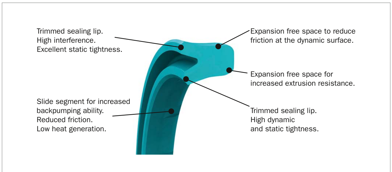
Figure 53: Zurcon® U-Cup RU9 design features
