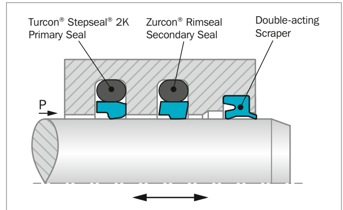
Figure 28: Zurcon® Rimseal in tandem configuration
