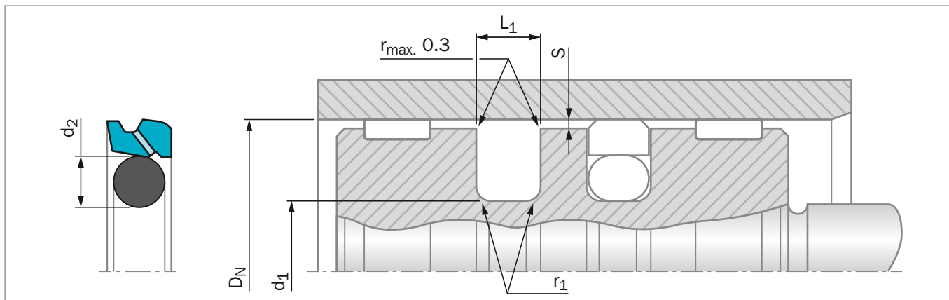
Figure 129: Installation Drawing
