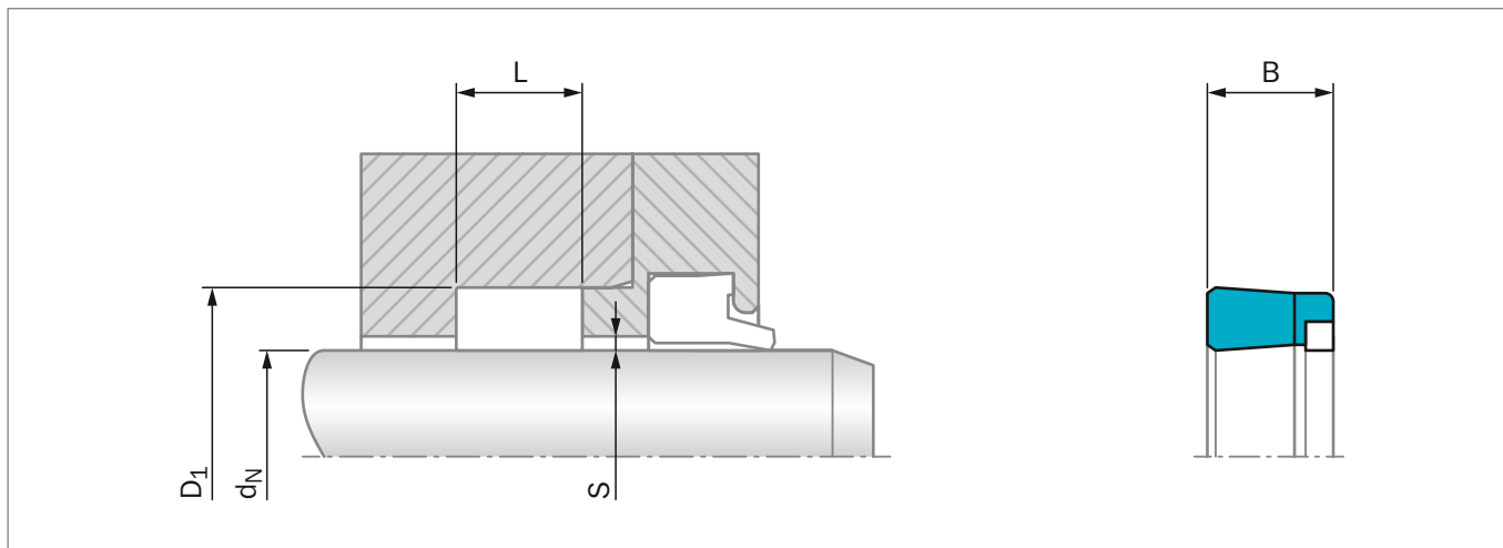
Figure 41: Installation Drawing
