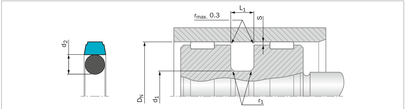
Figure 112: Installation Drawing
