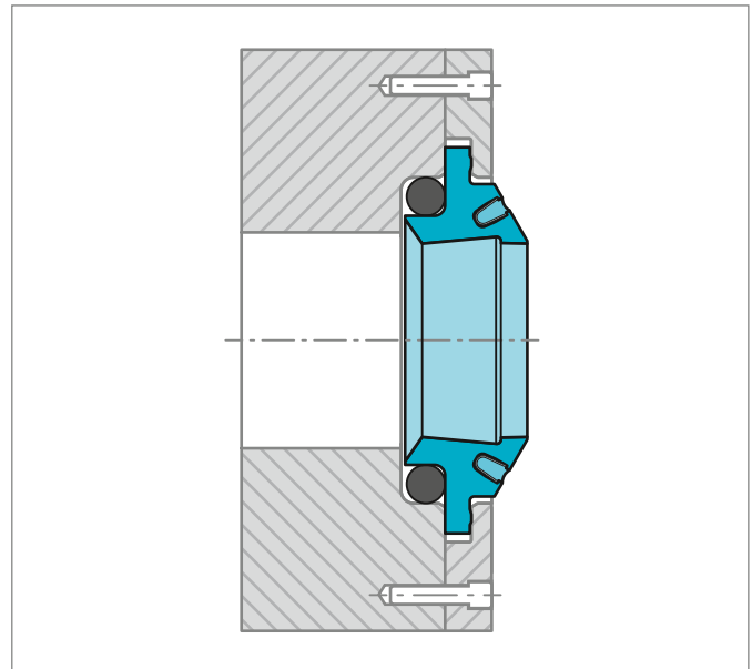
Figure 170: Turcon® Excluder® S installed in split groove
