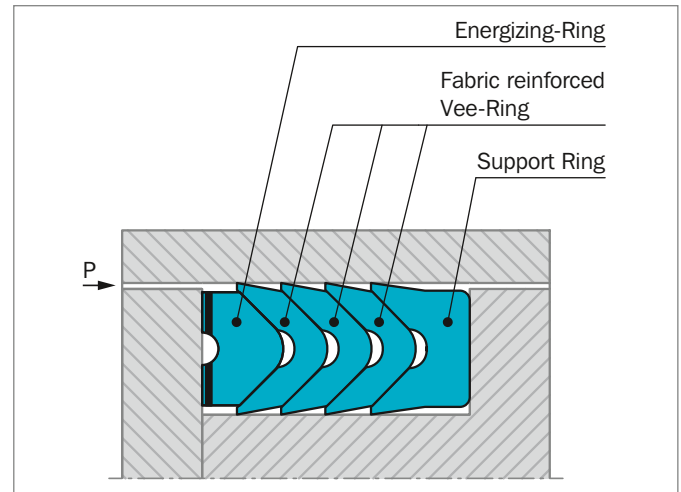
Figure 155: Veepac design with 3 fabric reinforced vee-ring
