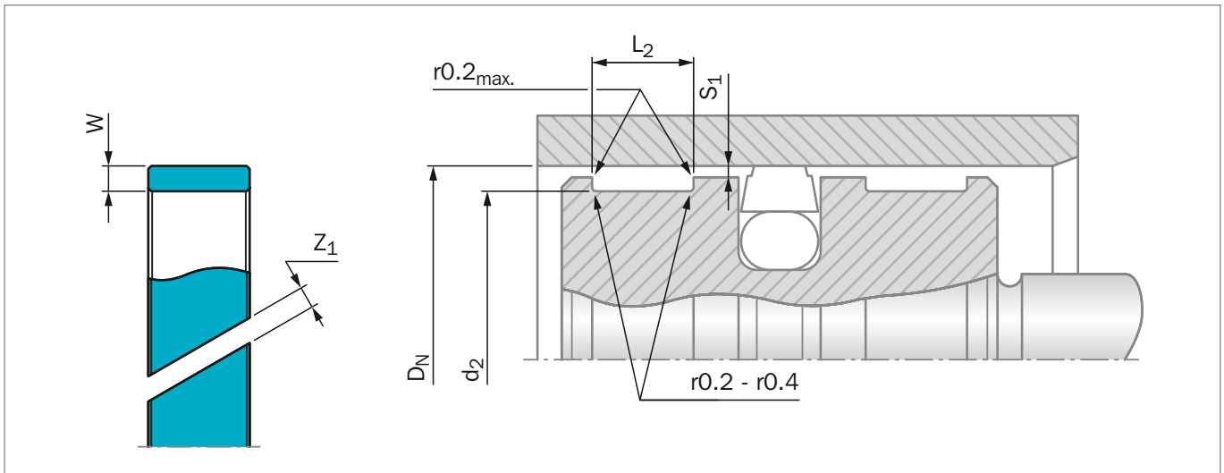
Figure 218: Installation Drawing
