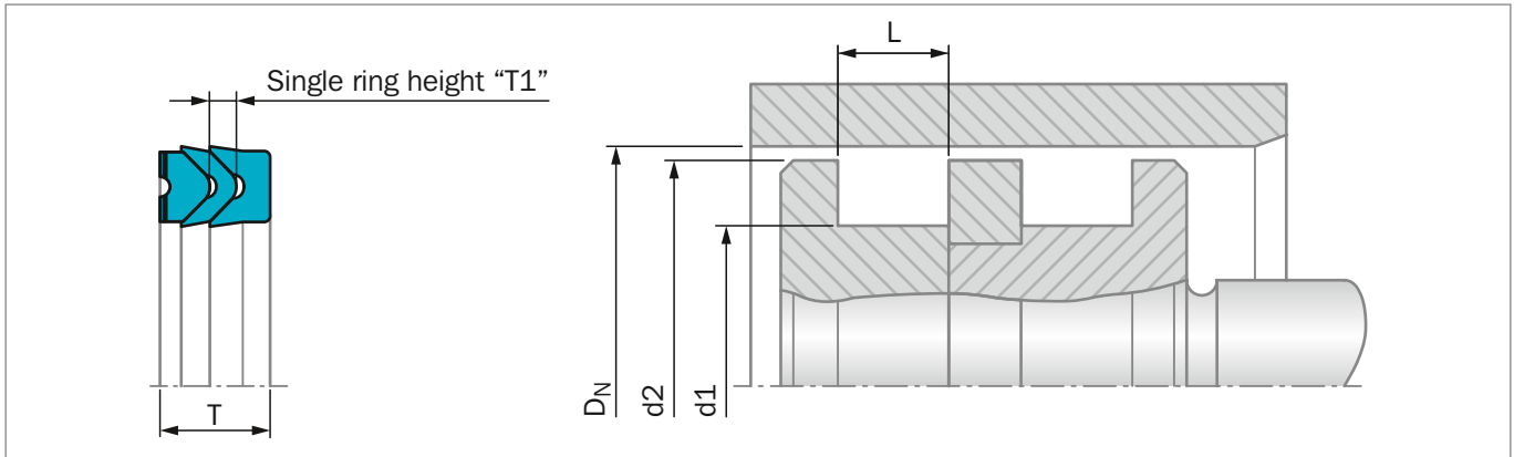
Figure 159: Installation Drawing
