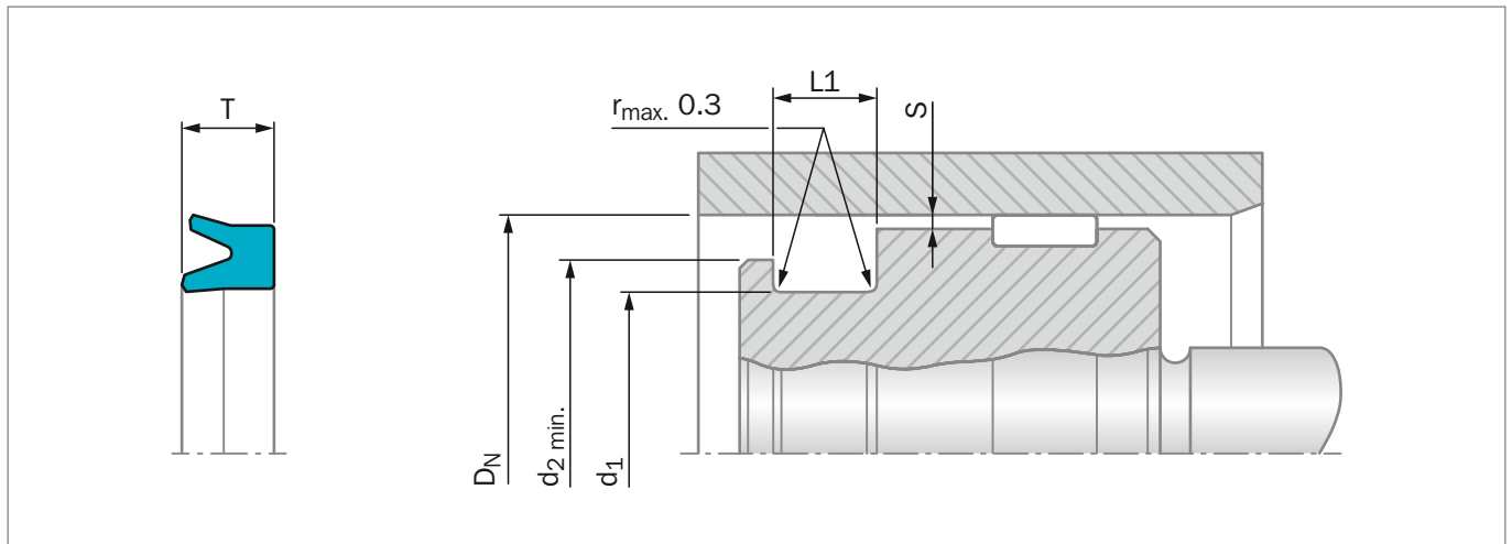
Figure 142: Installation Drawing
