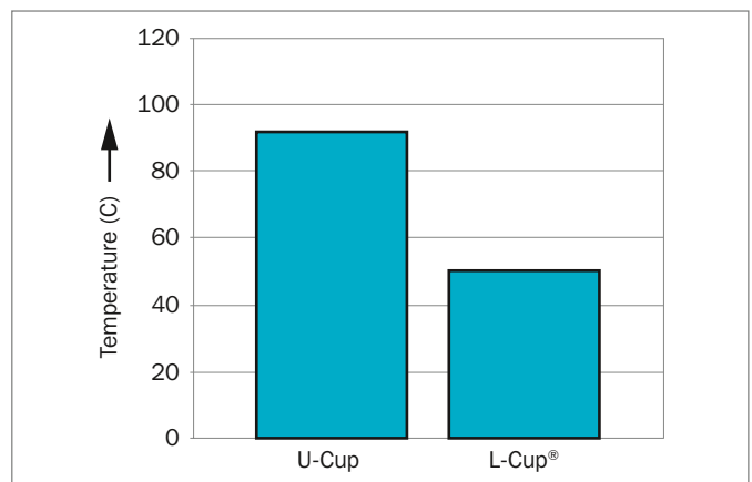
Figure 44: Increase in temperature caused by friction
