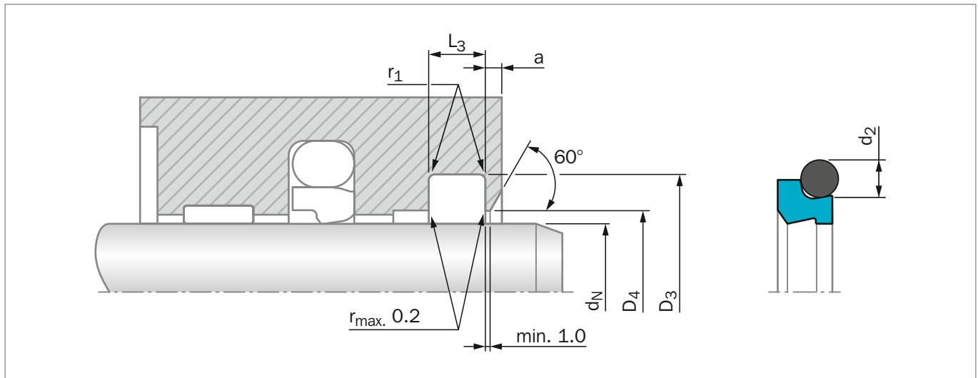
Figure 165: Installation Drawing
