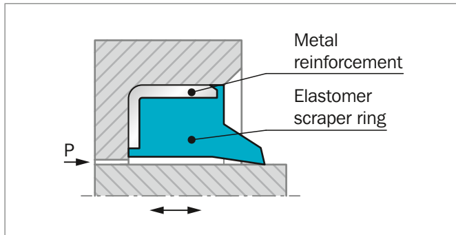
Figure 194: Scraper WSA
