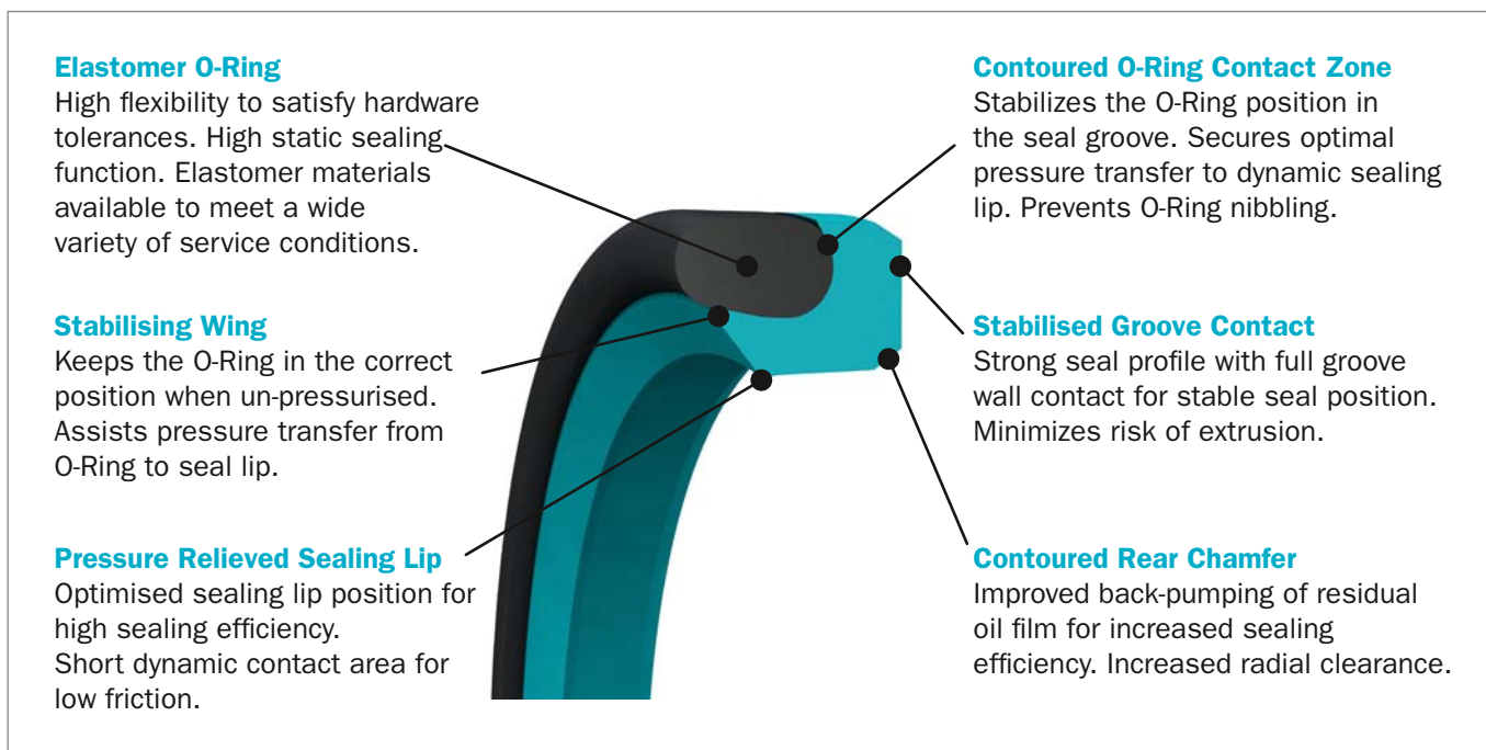
Figure 72: Turcon® VL Seal® design features
