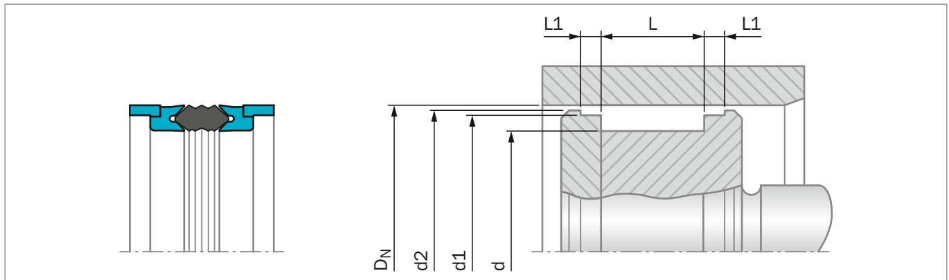
Figure 161: Installation Drawing
