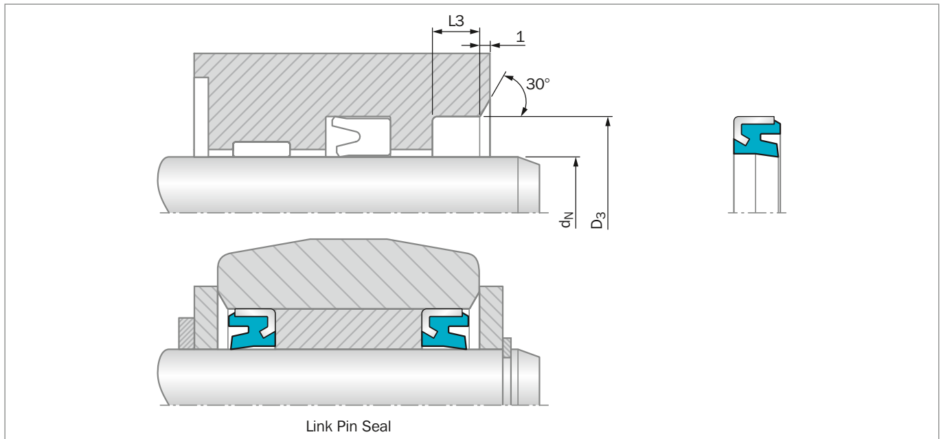
Figure 197: Installation Drawing
