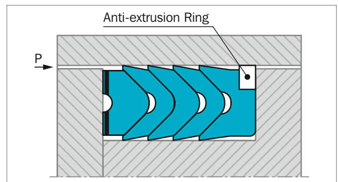
Figure 156: Veepac design with anti-extrusion ring
