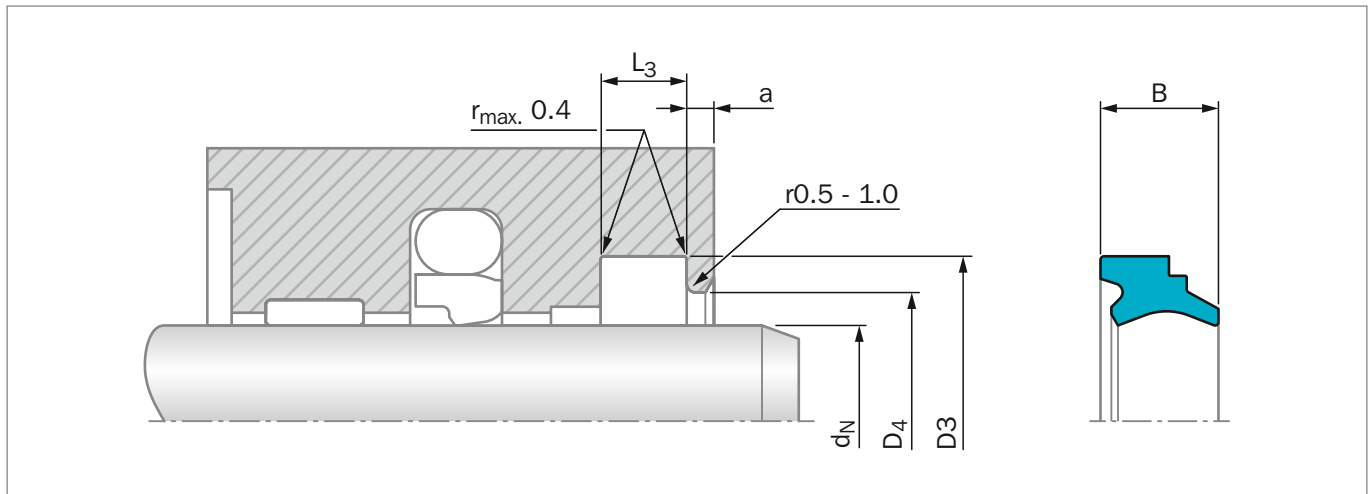
Figure 180: Installation Drawing
