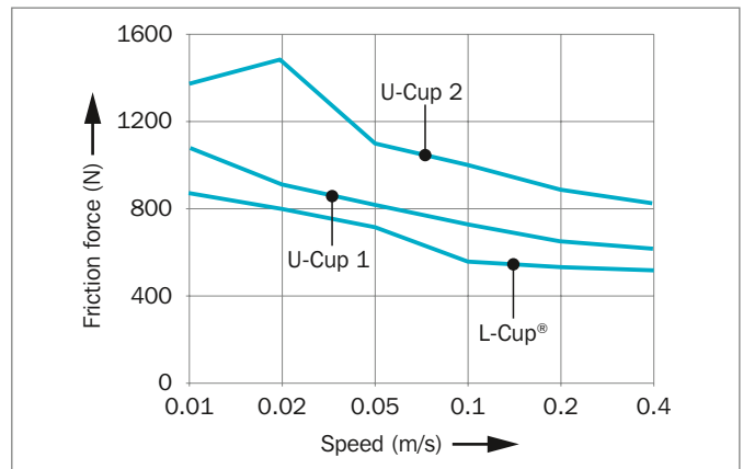
Figure 43: Friction dependent on speed
