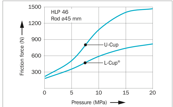
Figure 42: Friction dependent on pressure
