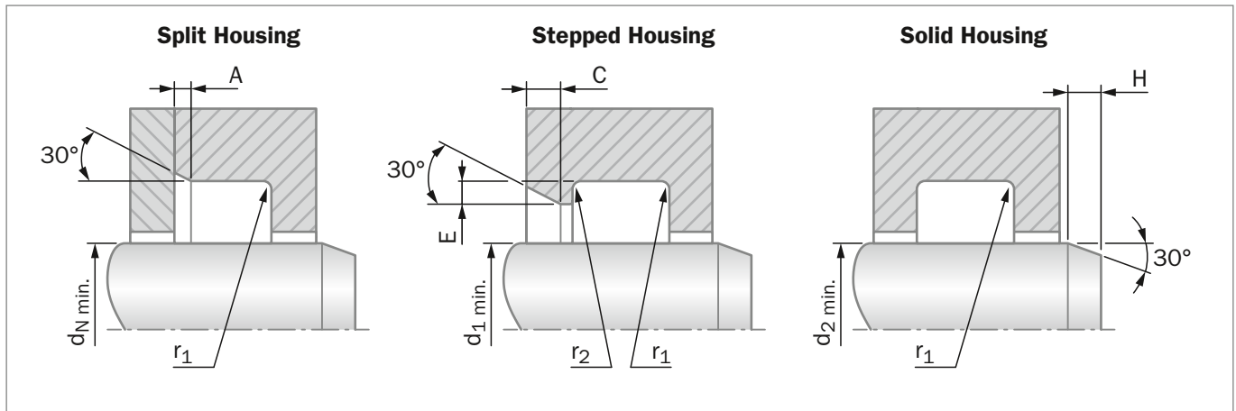
Figure 201: Variseal Groove Configurations
