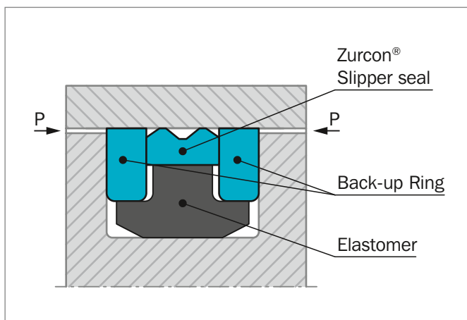
Figure 148: PHD/P Seal
