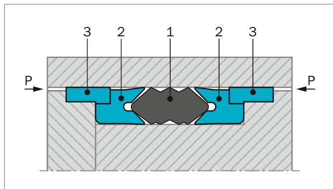
Figure 160: Selemaster design
