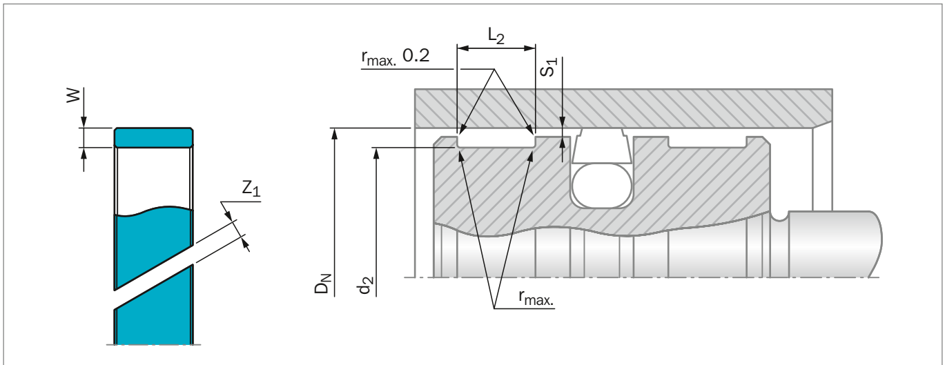
Figure 213: Installation Drawing
