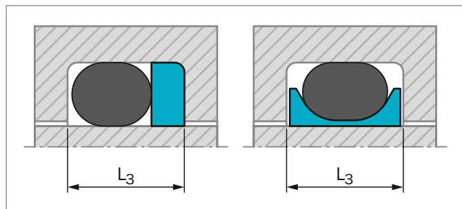
Figure 94: Groove width
