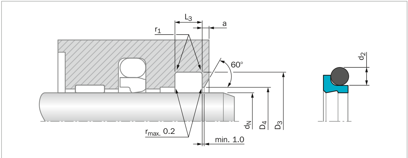
Figure 163: Installation Drawing
