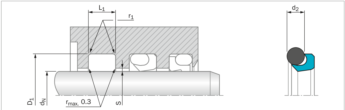
Figure 74: Installation Drawing
