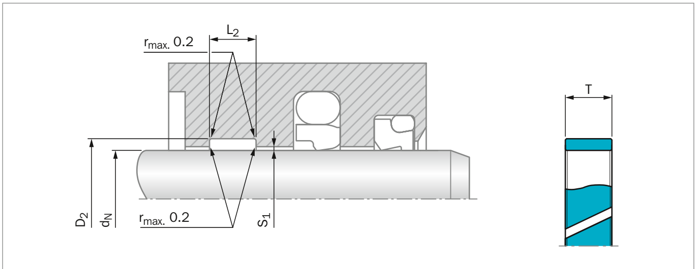
Figure 206: Rod guide
