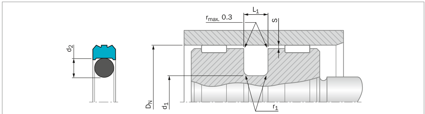
Figure 147: Installation Drawing
