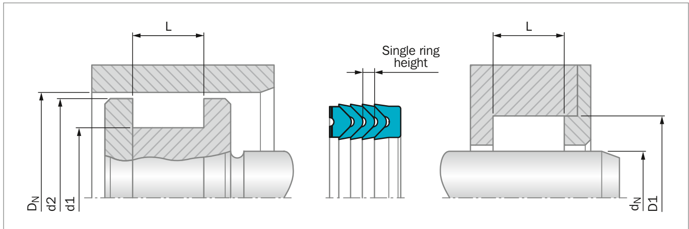
Figure 157: Installation Drawing
