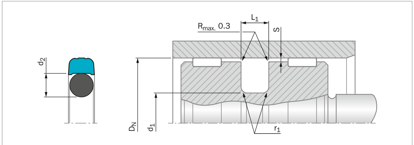
Figure 117: Installation Drawing
