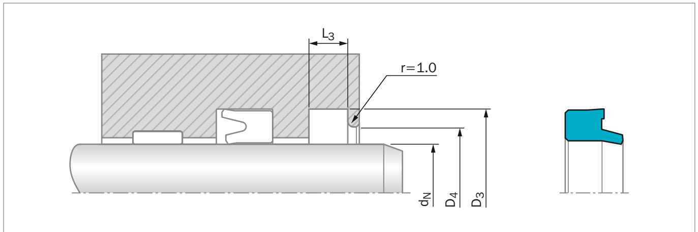
Figure 191: Installation Drawing
