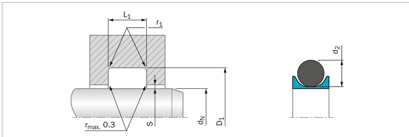
Figure 93: Installation Drawing
