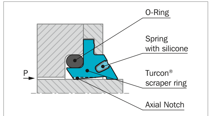
Figure 172: Optional Turcon® Excluder® SN where internal sealing lip has axial notch.
