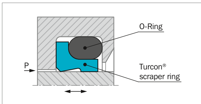
Figure 162: Turcon® Excluder® 2
