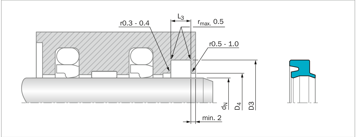
Figure 182: Installation Drawing
