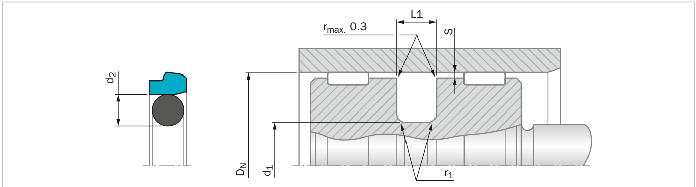
Figure 126: Installation Drawing
