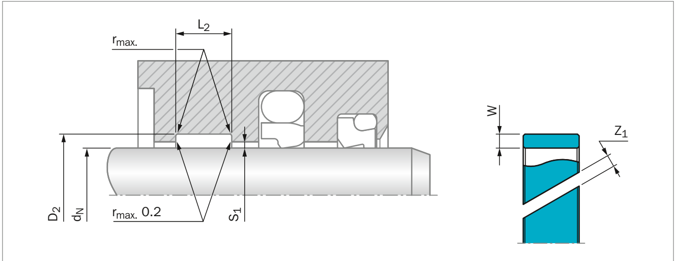
Figure 215: Installation Drawing
