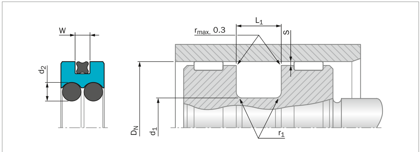
Figure 122: Installation Drawing
