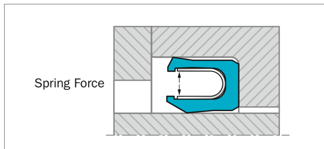
Figure 67: Turcon® Variseal® without system pressure
