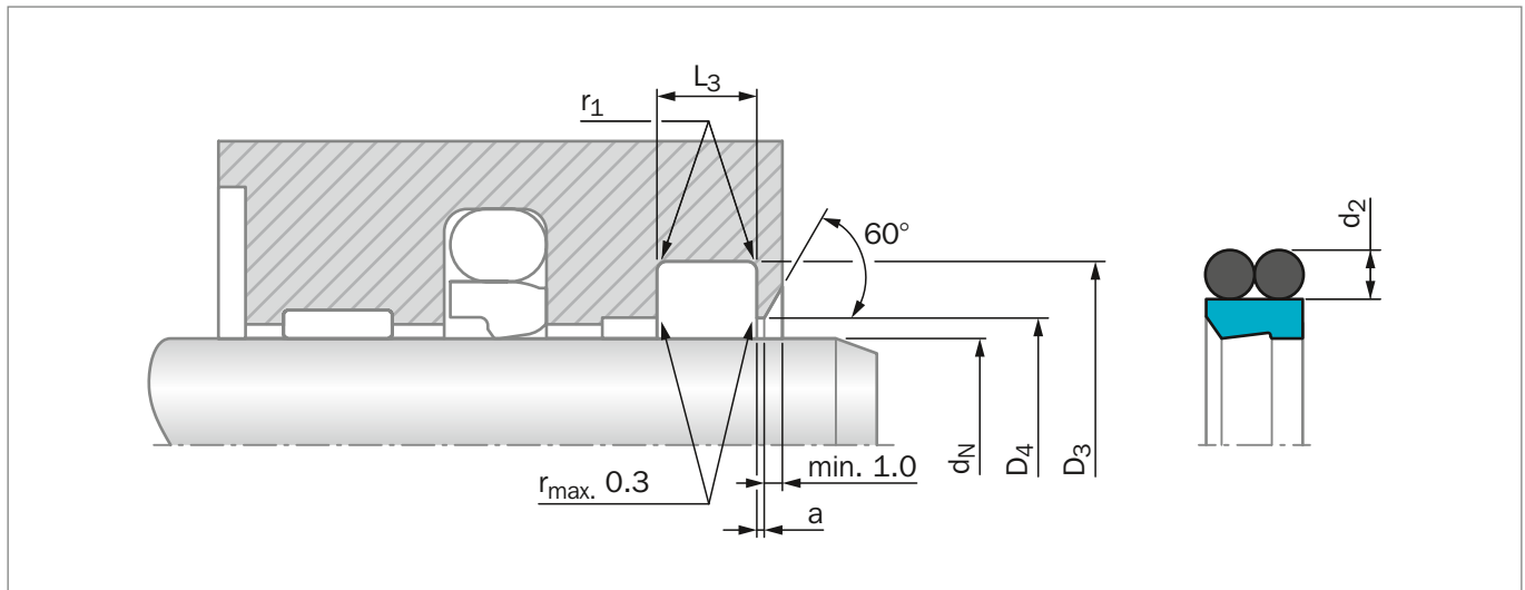
Figure 167: Installation Drawing
