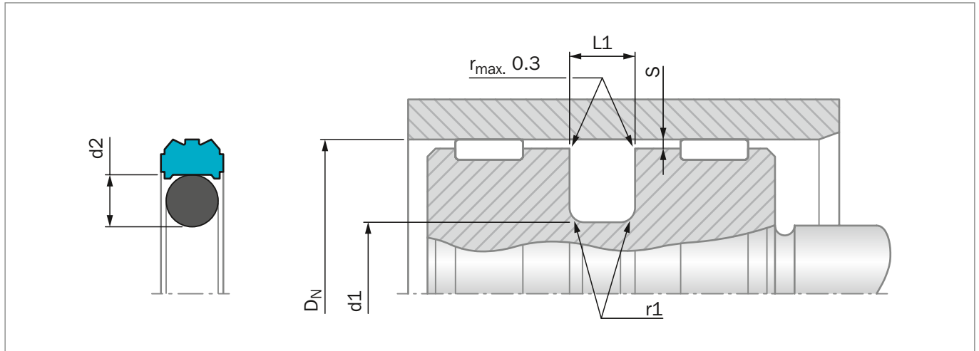
Figure 144: Installation Drawing
