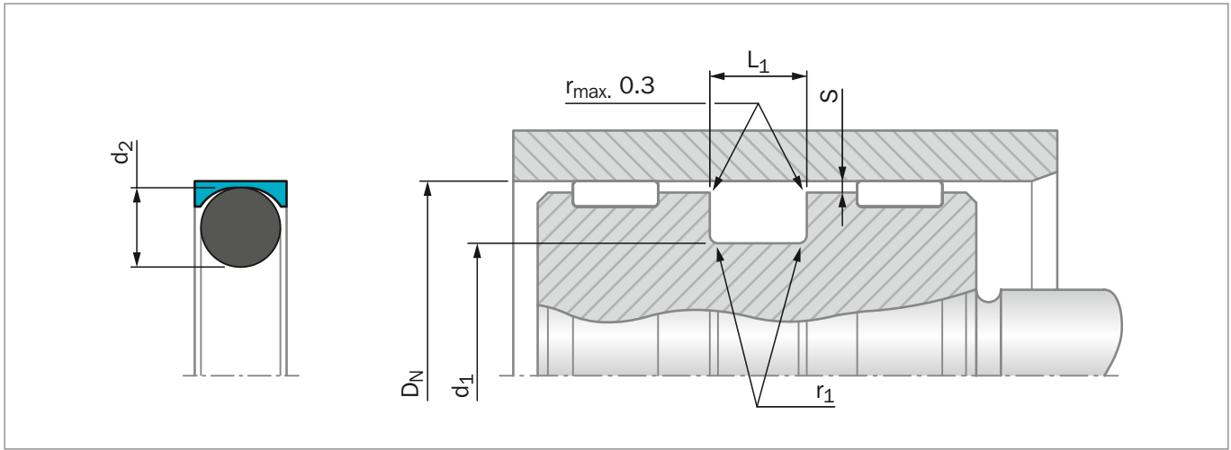
Figure 132: Installation Drawing
