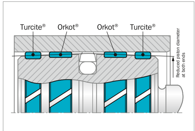
Figure 217: Arrangement of the Slydring® on the piston
