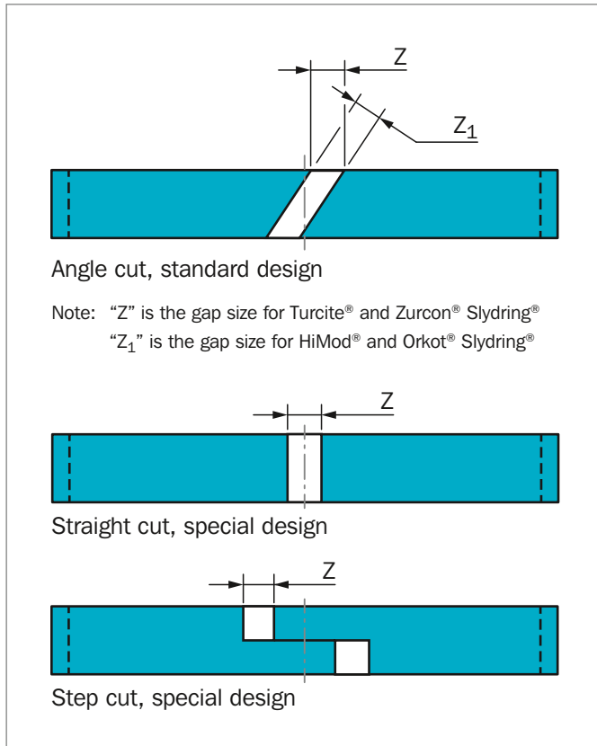
Figure 203: Type of cut
