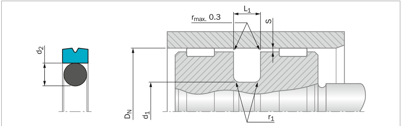
Figure 115: Installation Drawing
