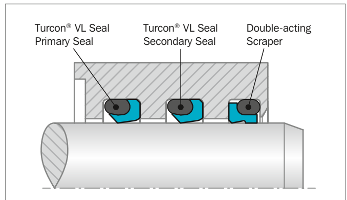
Figure 73: Turcon® VL Seal® in tandem configuration
