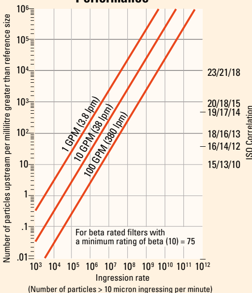
Flow Rate Effect on Off-Line Filtration Performance
