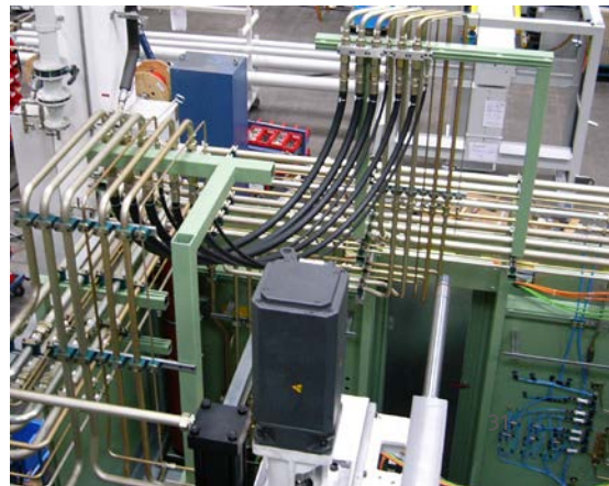
Fig. 11 Pipeline routing in a large machine
