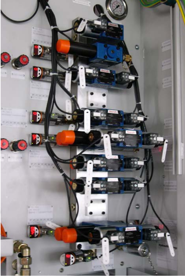
Fig. 20 Marking hydraulic valve blocks
