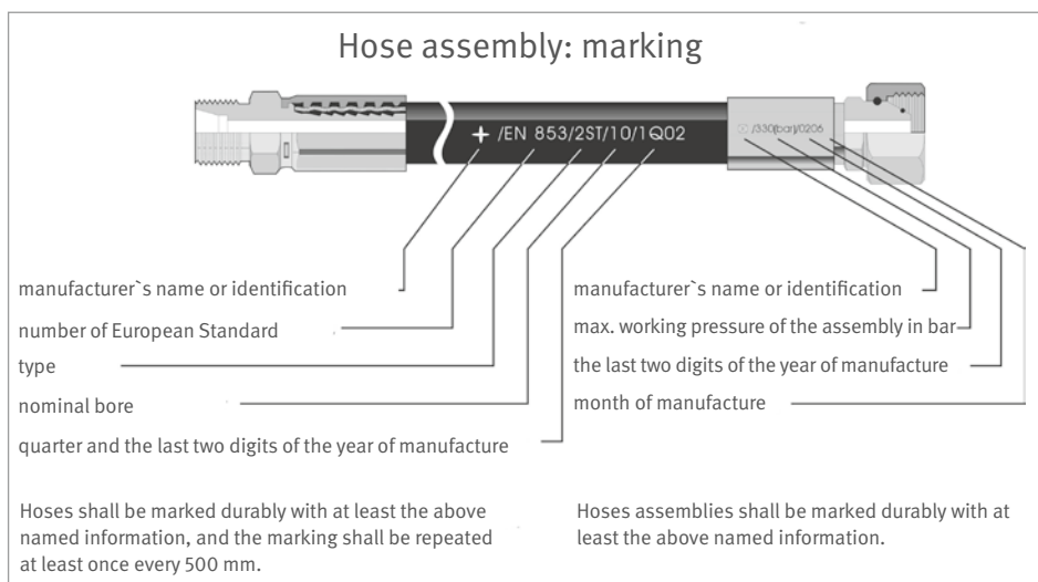
Fig. 13 Structure and labeling of a hose assembly
