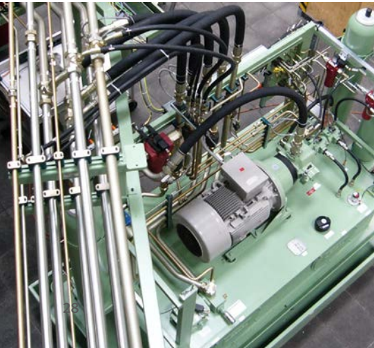
Fig. 9 Central hydraulic system at commissioning
