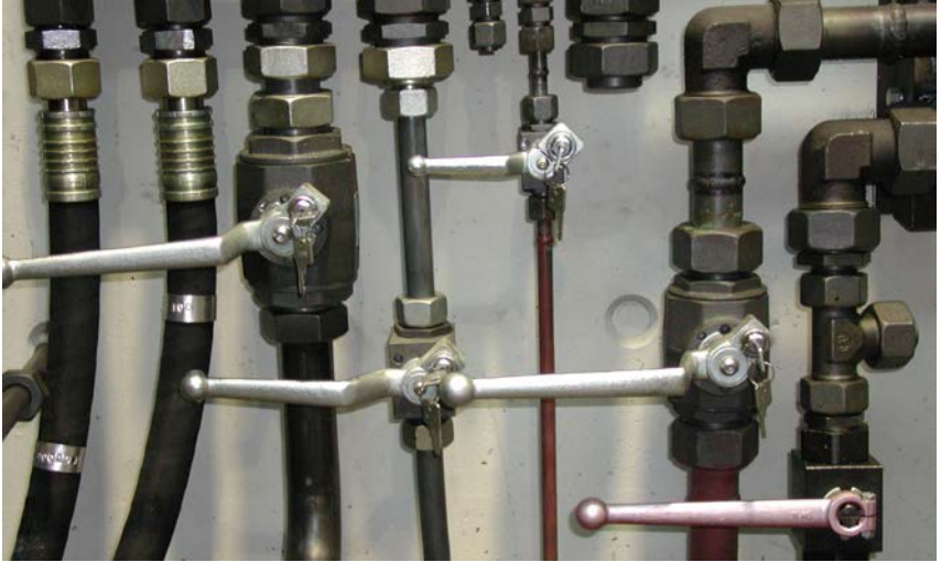
Fig. 3 Securing against unintentional re-closing by lockable ball valves.
