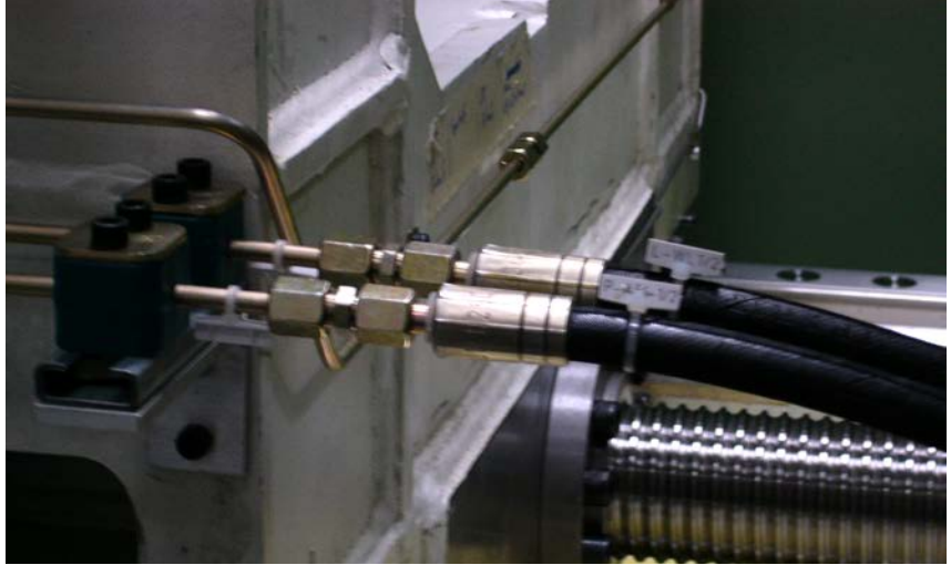
Fig. 26 Markings on pipe and hose side
