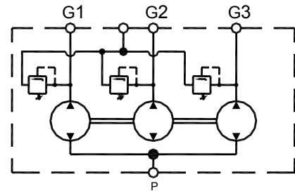
Diagram Of Three - Element Divider With Motor
