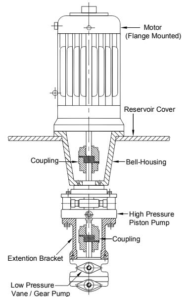
Assembly of Motor , Bell - Housing , Piston pump , Extension Bracket And Low Pressure Pump
