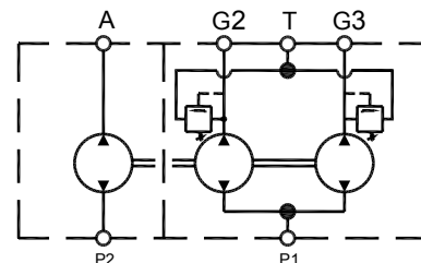
Diagram Of Two - Element Valve With Motor
