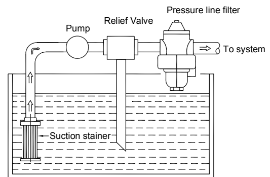
SYSTEM USING PRESSURE LINE FILTER
