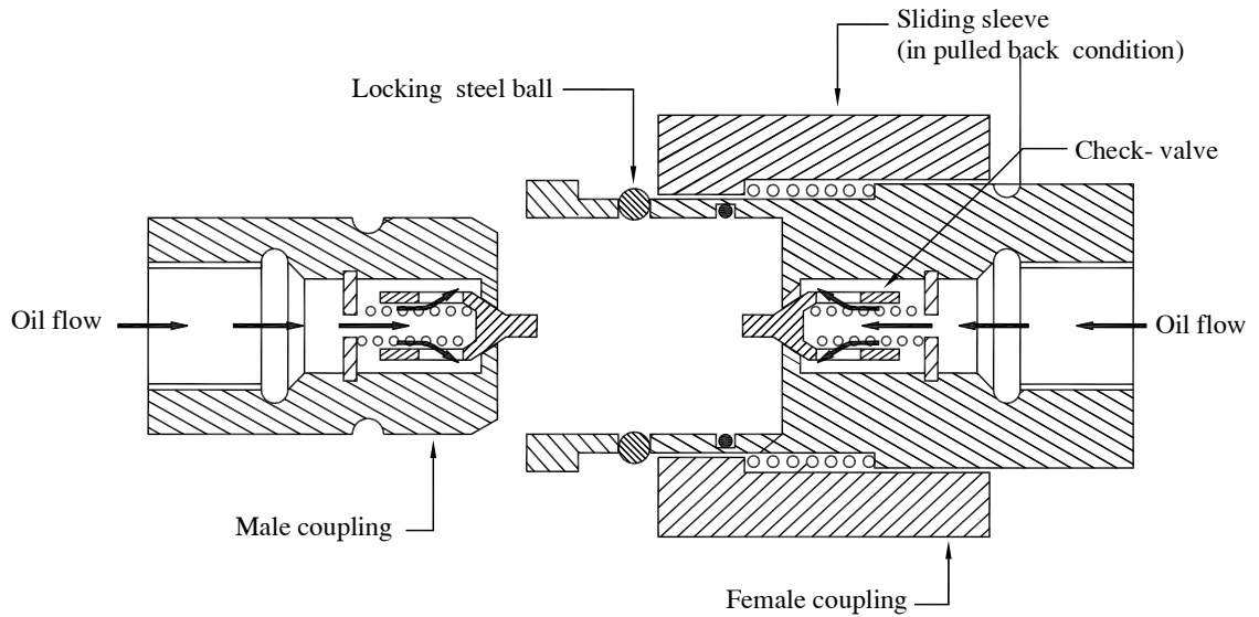
Quick-connection coupling
