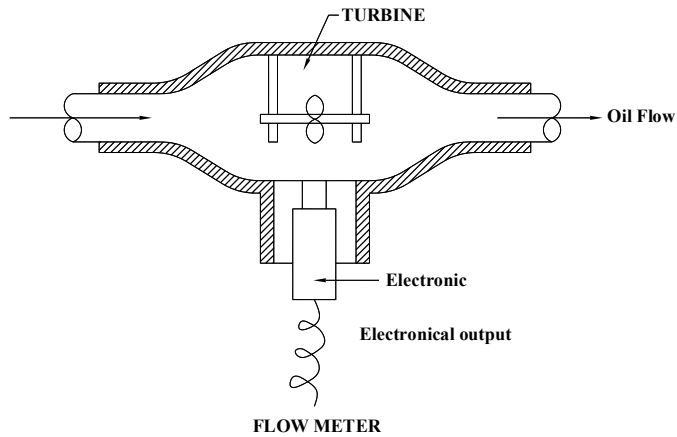
Turbine Meter Mfg. by:- webster-instruments
