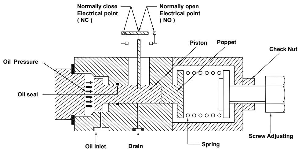
Pressure Switch (Skematic Diagram)
