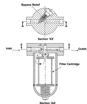
Cross section of pressure line filter
