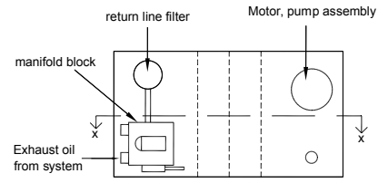
Top view of power unit with wave-system baffle configuration
