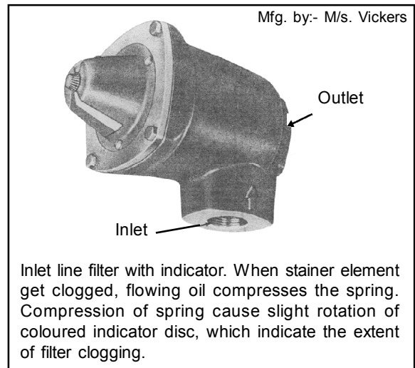
Inlet line filter connected before pump outside tank. (A 100 mesh size strainer can protect pump from particals upto 150 micron size)
