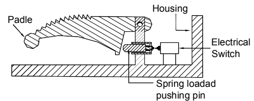
Cross-section of foot operated switches
