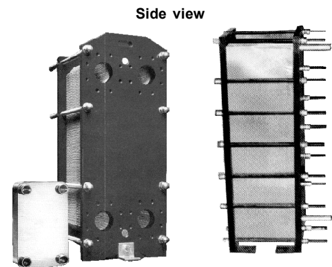
Plate type Heat Exchanger Mfg. by:- M/s. Ind Swep Energy Systems, Pune
