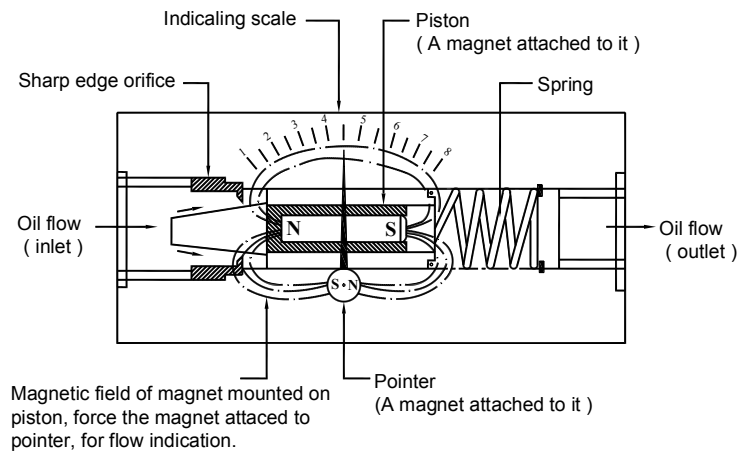
Orifice type of Flow Meter Mfg. by:- webster-instruments
