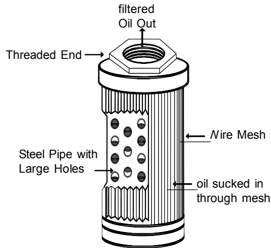
IN-TANK SUCTION STAINER
