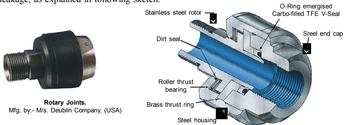
Rotary Joints. Mfg. by:- M/s. Deublin Company. (USA)
