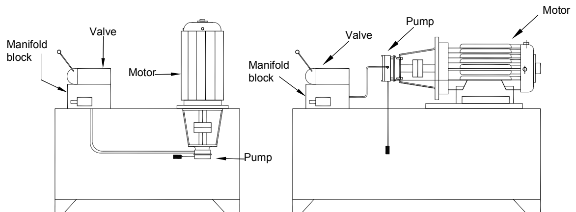
Tank top assembly type reservoir
