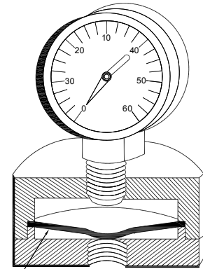
Diaphragm Diaphragm protected gauge
