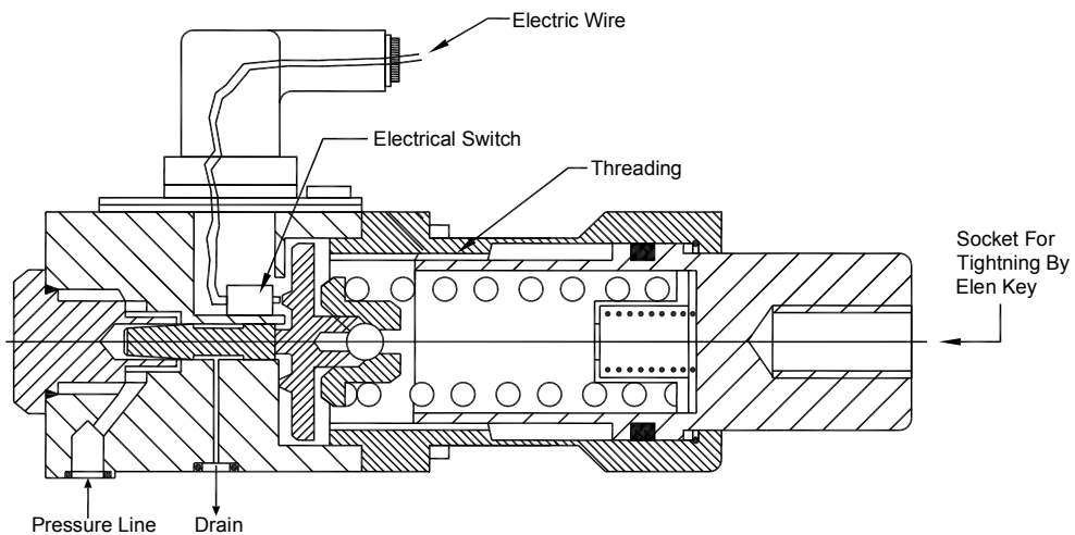
Cross Section of - Model _____ Presure Switch of M/S Polyhydron
