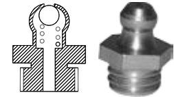
Grease Nipple Mfg. by:- www.rbrhw.com
