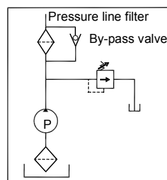
HYDRAULIC CIRCUIT DIAGRAM USING PRESSURE LINE FILTER
