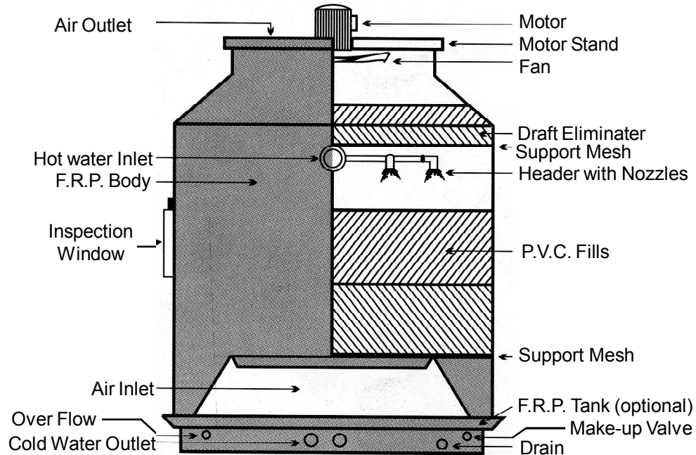
F.R.P. COOLING TOWER Mfg. by M/s.National Engineering
