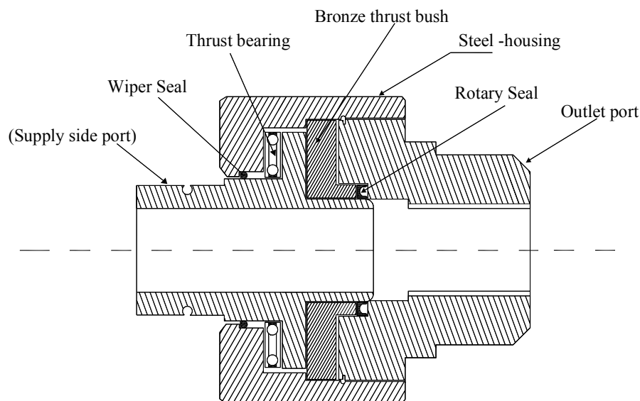
Rotary Joints. Mfg. by:- M/s. Deublin Company. (USA)
