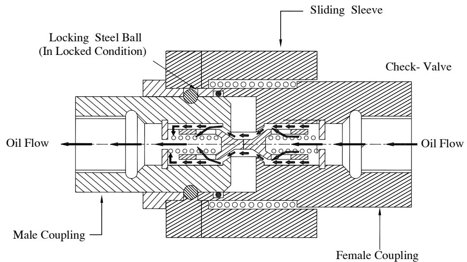
Quick - Connection Coupling
