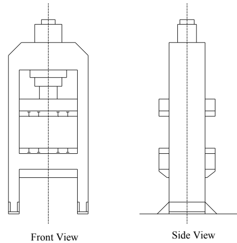
Figure No. 4.6, H-Frame Press
