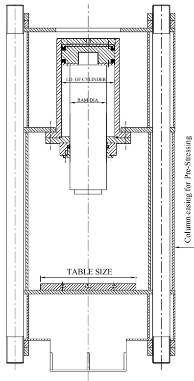
FOUR COLUMN DOWN STROKE HYDRAULIC PRESS WITH DOUBLE ACTION CYLINDER
