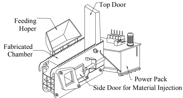
Figure No. 4.12, Scrap Bailing Press
