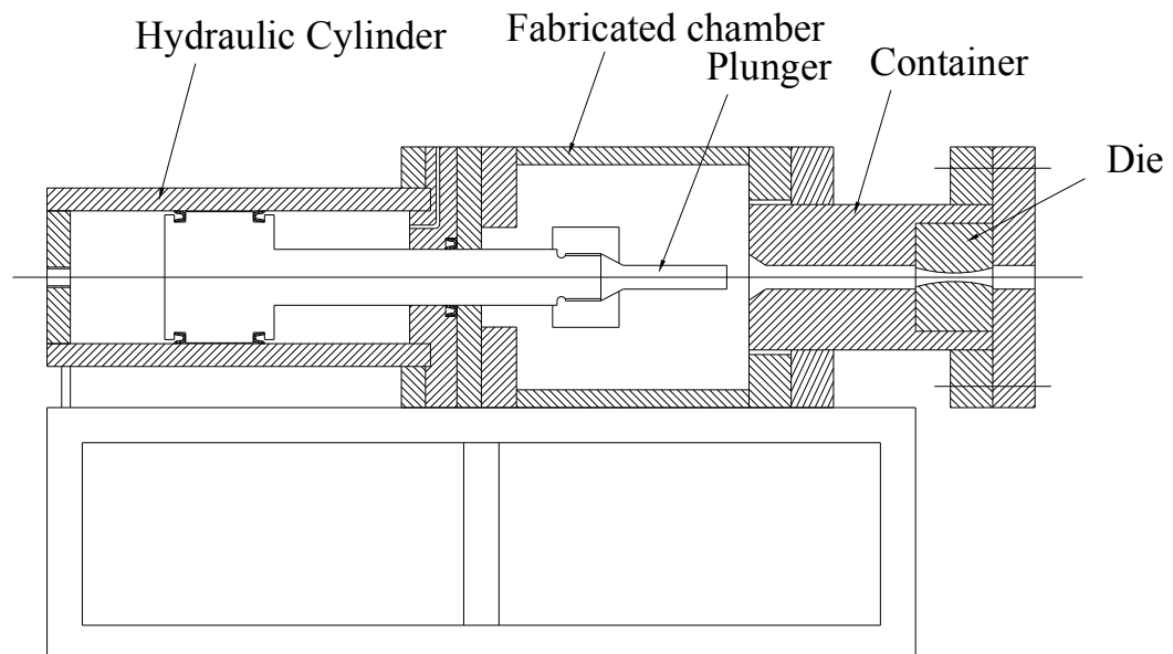
Figure No. 11 Extrusion Press
