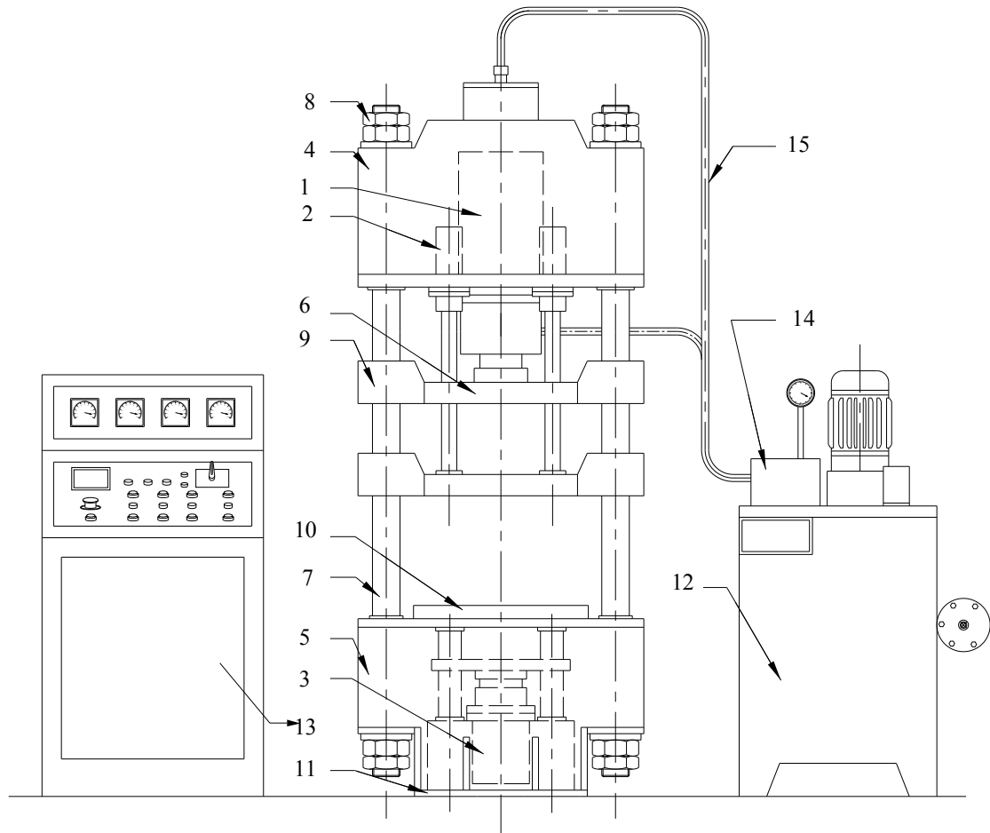
FIGURE NO.1.1, HYDRUALIC PRESS
