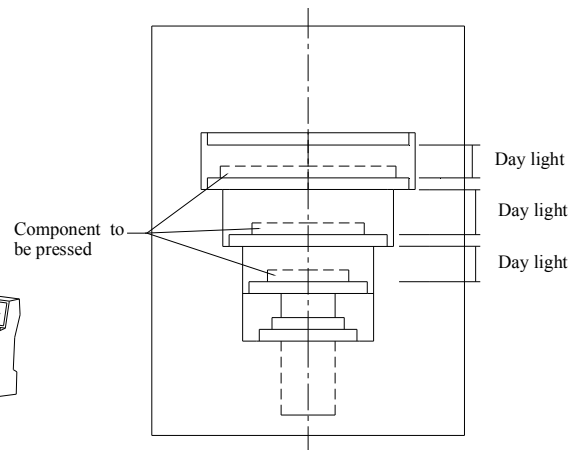
Figure No. 3.4, Three Day-light Press
